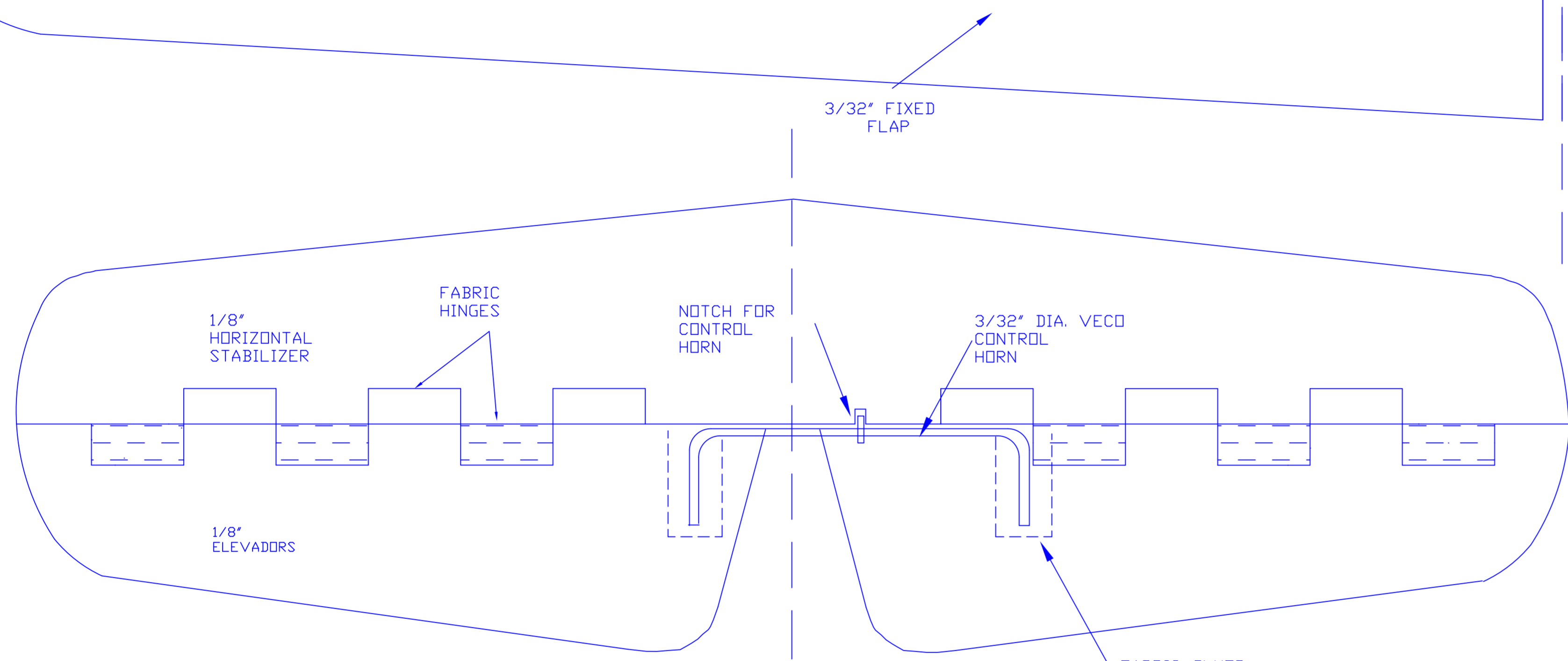
HORIZONTAL STABILIZER TOP VIEW
